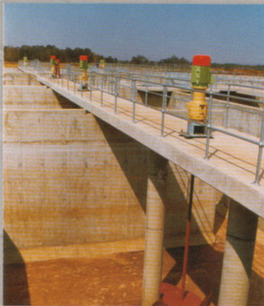
Large Anaerobic Basin Application
