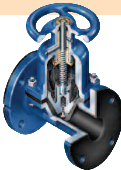
Dia-Flo Rubber Lined Valve
